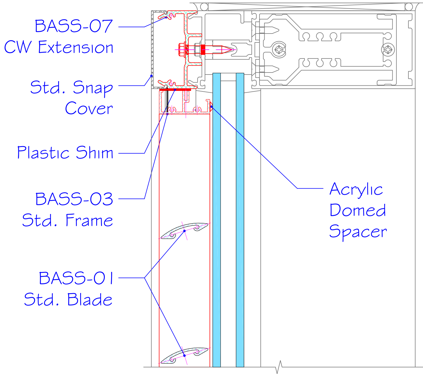
(A) BASS @ Curtain Wall Head
